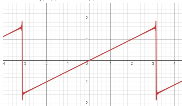
S_{f,n}(t) when f(t) = t , n = 500
