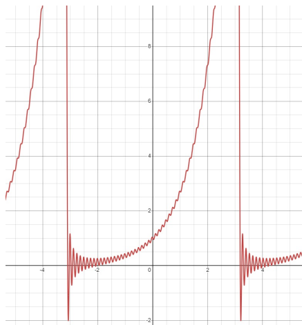
S_{f,n}(t) when f(t) = e^t , n = 50
