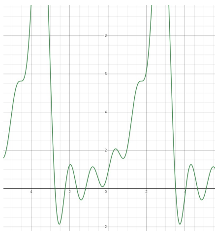
S_{f,n}(t) when f(t) = e^t , n = 5
