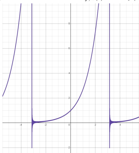
S_{f,n}(t) when f(t) = e^t , n = 500
