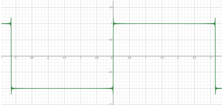
S_{f,n}(t) when f(t) = \text{sgn}(t) , n = 500
